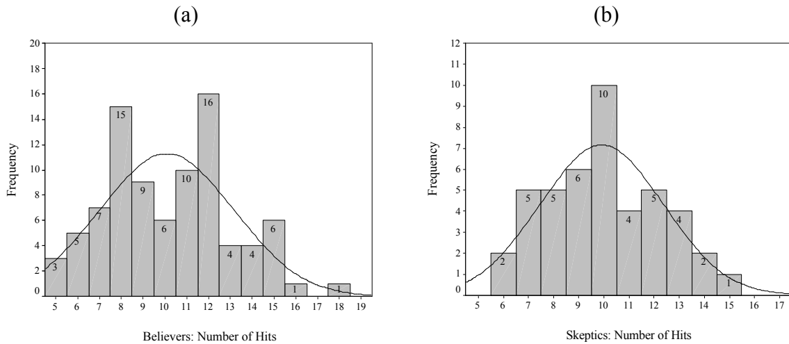
Fig. 3. (a) For believers ( n = 87 ), scoring deviated marginally significantly from a normal distribution, which included a prominent deficit in scores at MCE = 10 . (b) For skeptics ( n = 44 ), scoring followed a normal distribution, although scoring at MCE was very high.
